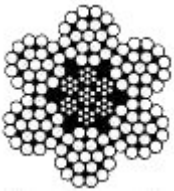
6 x 19 (1 + 6 + 12) WITH IWRC
